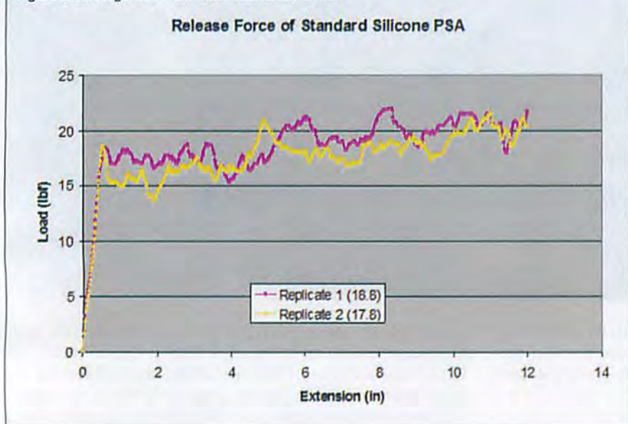
Figure 2. Average 180° Peel Test Results for a PSA
